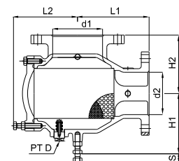
FLANGED TYPE
