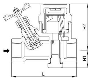
Type YSP-1 (Bypass valve attached)
